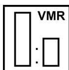
VMR - Volume Mixing Ratio
